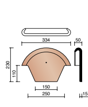
P000 1240 Fronton 230 mm
